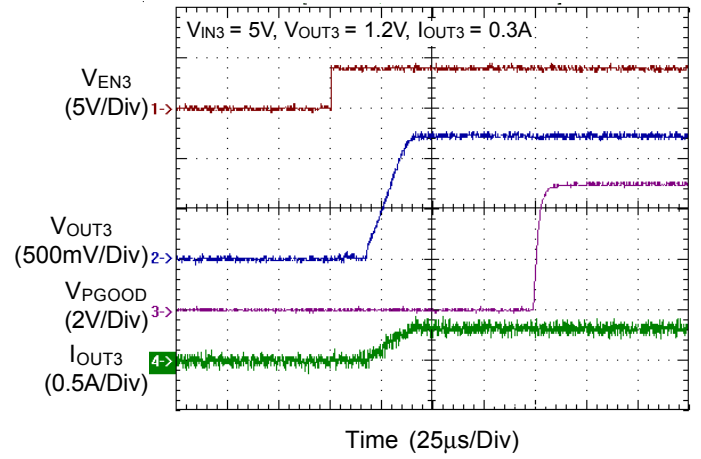
LDO2 PGOOD Response
