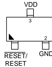
SOT-23-3 (L-Type)
