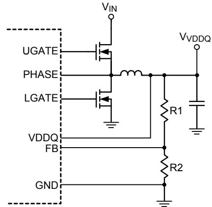
Figure 6. Setting VDDQ with a Resistive Voltage Divider
