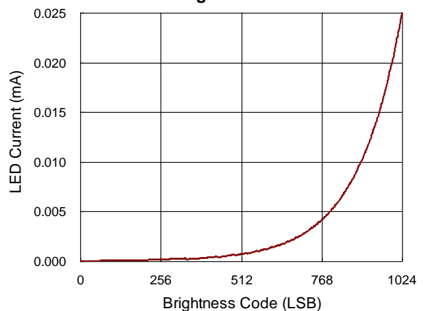
10 bit LED Current vs. Exponential Brightness Code
