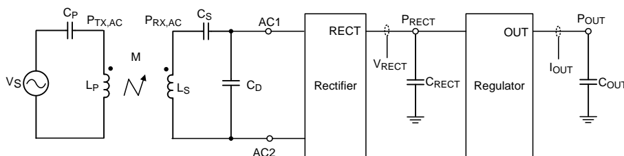
Figure 13. Received Power Sensed
