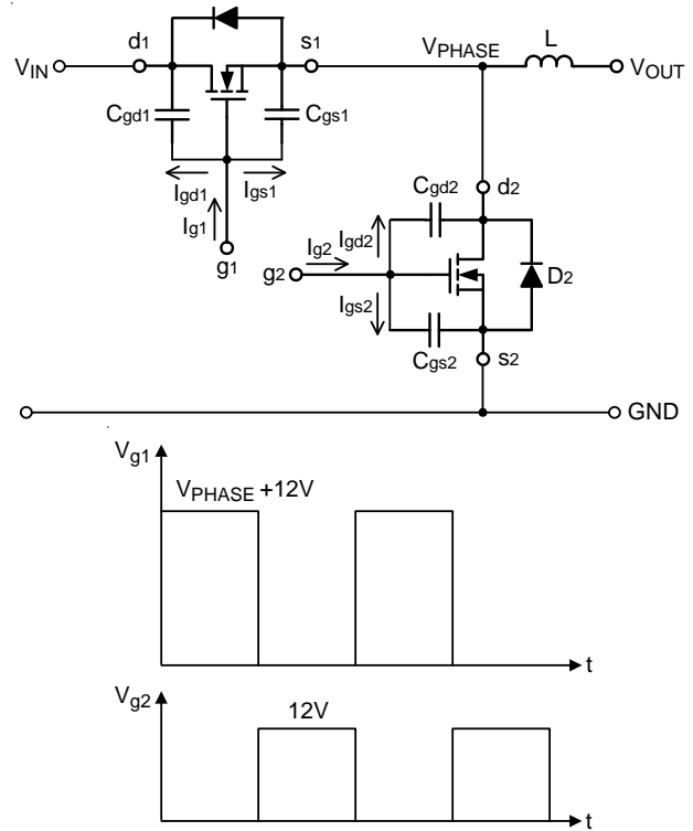
Figure 2. Equivalent Circuit and Waveforms ( V_{CC} = 12V )
