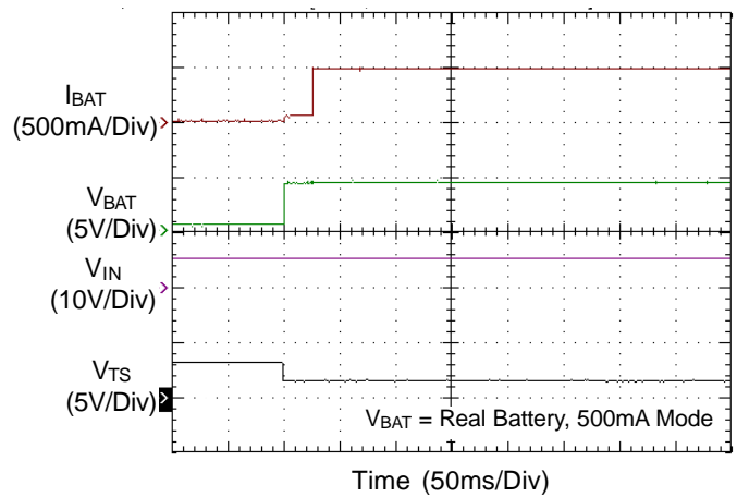
Battery with NTC Resistor Plug-In
