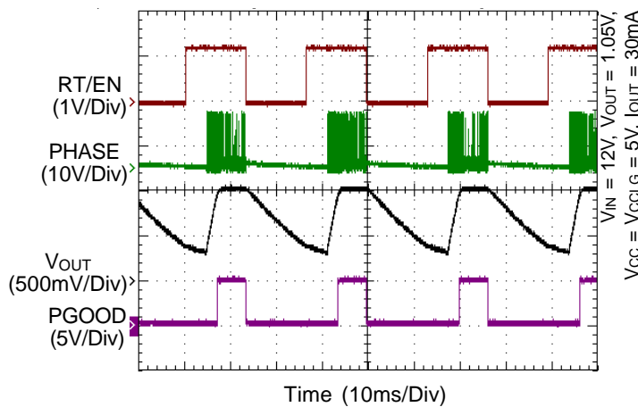
Pre-Bias Startup
