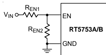
Figure 8. Resistive Divider for Under-Voltage Lockout Threshold Setting
