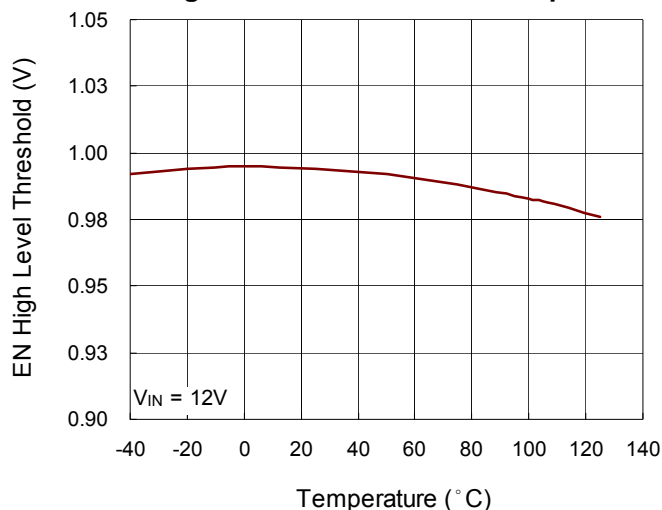
EN High Level Threshold vs. Temperature
