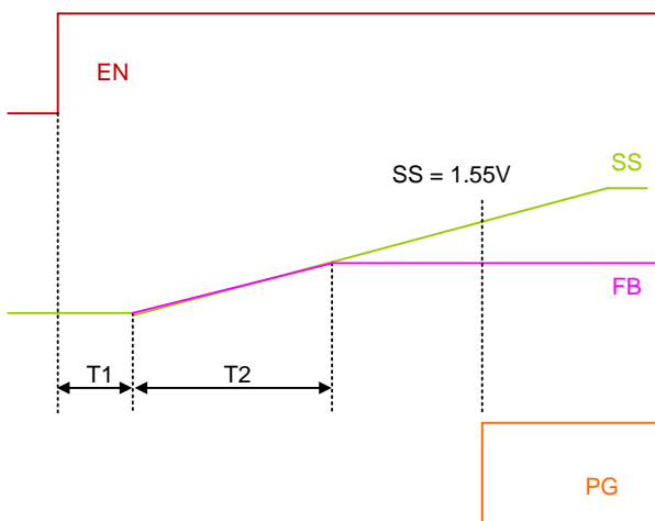
T1 : EN delay, from EN go high to SS start rising, T1 = 50μs; T2 : normal SS, from FB rising to settled, T2 = C SS × 0.9/I SS ; PG go high after SSOK (SS = 1.55V)
