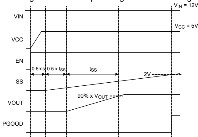
Figure 1. Start-Up Sequence
