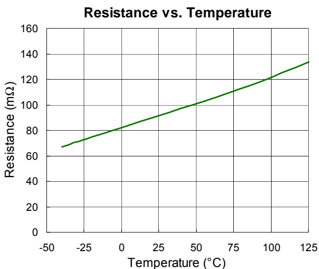
Figure 15. RTQ2106 R_{DS(ON)} vs. Temperature
