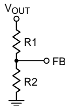
Figure 4. Setting V OUT with a Resistive Voltage Divider
