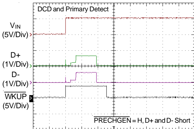
Time (100ms/Div)
