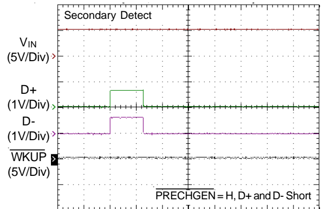
Time (100ms/Div)
