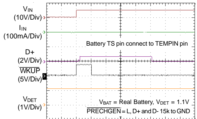
Time (250ms/Div)
