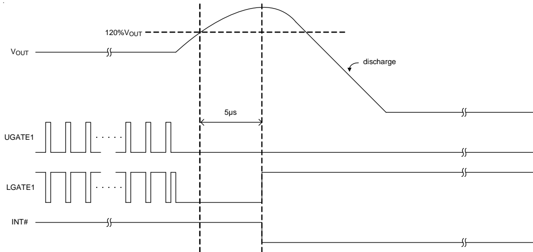
Figure 6. OVP Behavior
