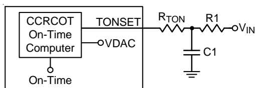
Figure 11. VDD Controller : On-Time Setting with R_C filter
