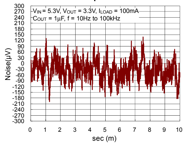
Output Noise
