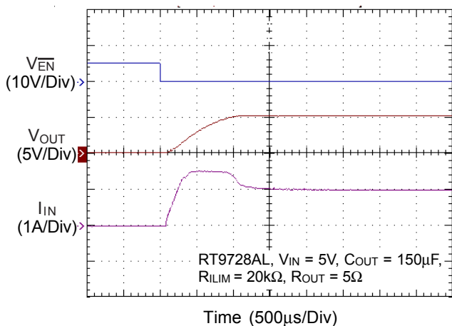
Power On from \overline{\text{EN}}
