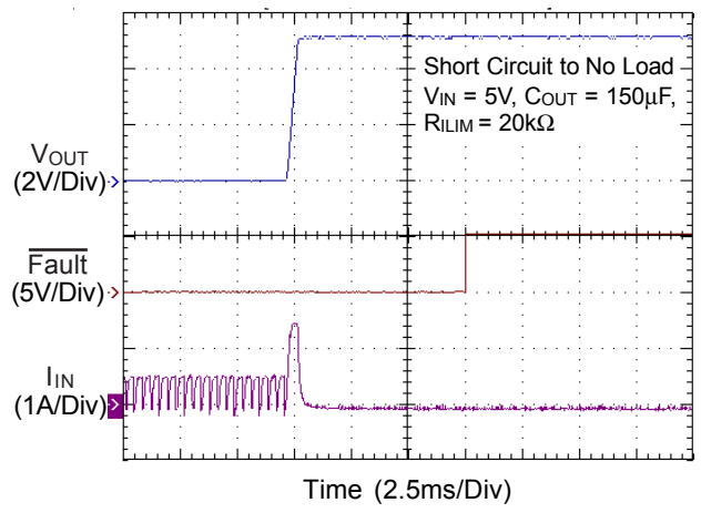
Current Limit
