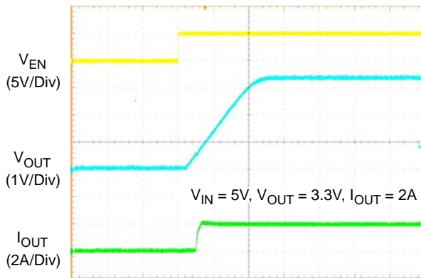
Time (500µs/Div)
