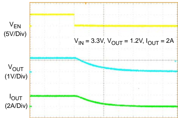
Time (10µs/Div)
