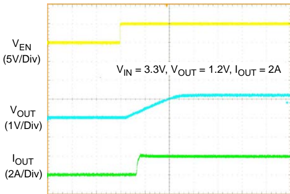
Time (500µs/Div)
