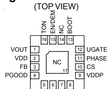
RT8209L WQFN-16L 3x3
