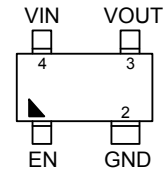
SC-82 (SSOT-24)
