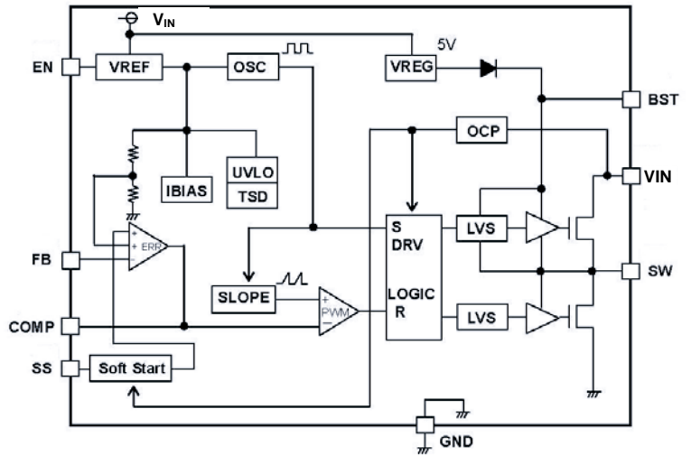
Figure 3. Block Diagram
