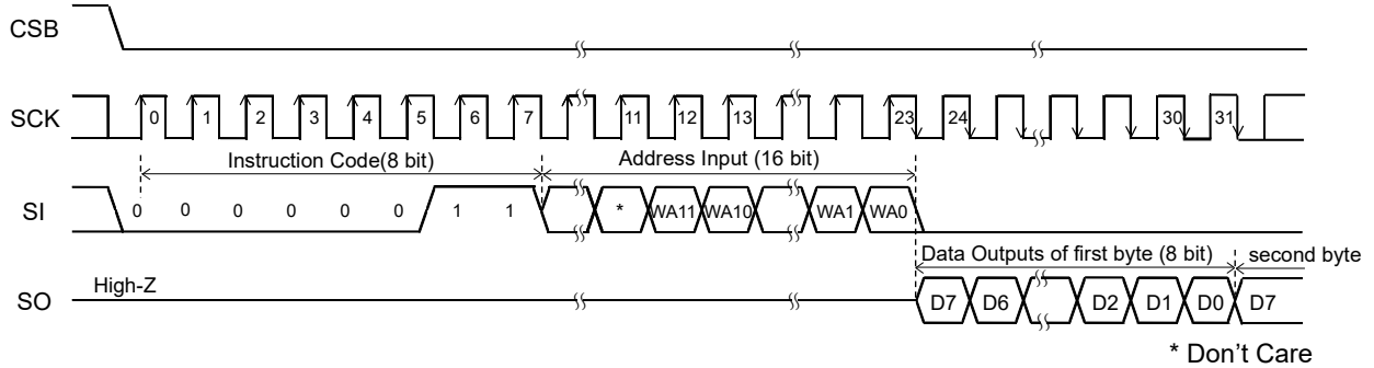
Figure 41. Read Command
