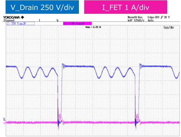
Figure 11. V_{in\_dc} = 900\text{ V} , I_o = 0.5\text{ A} Primary Side
