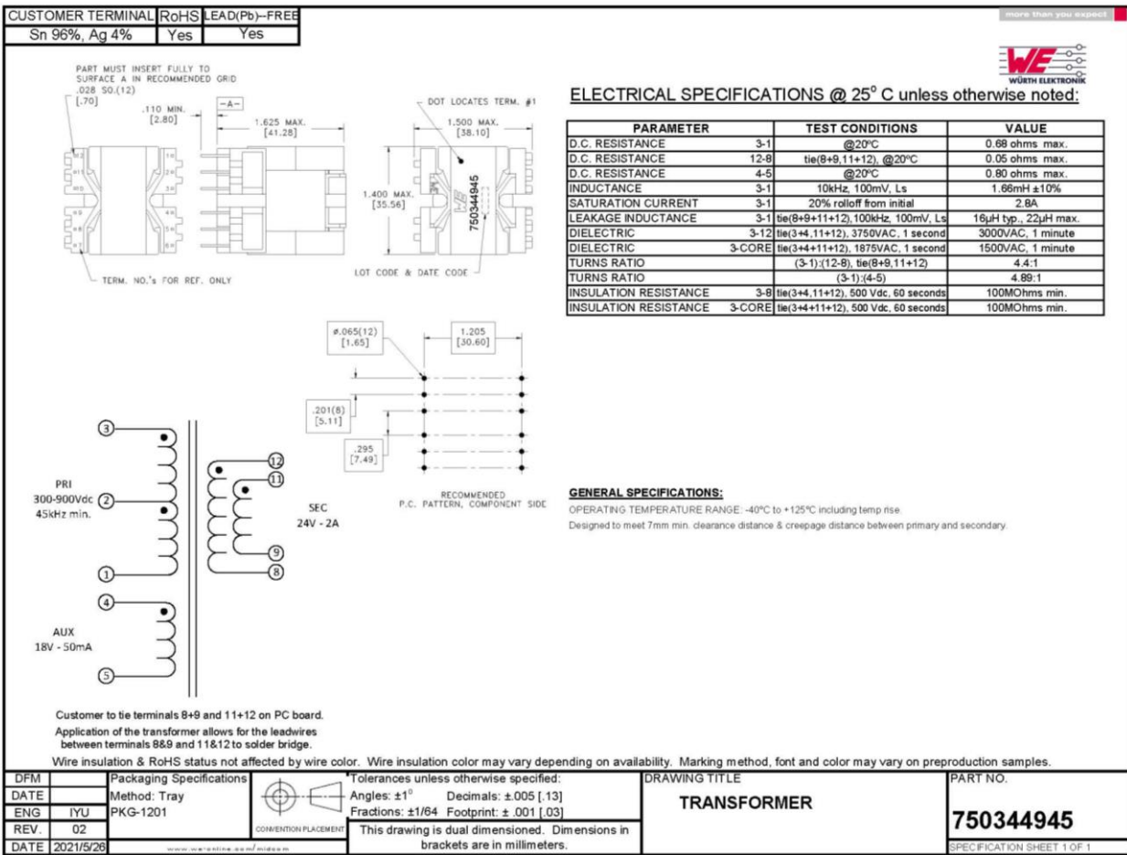
Figure 5. Transformer Specification
