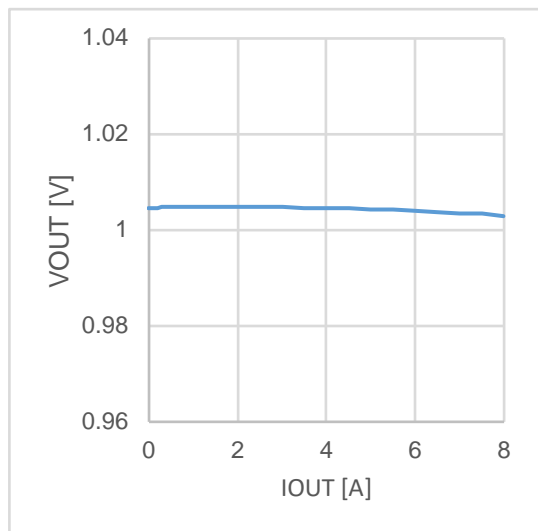
Figure 11. Load Regulation
