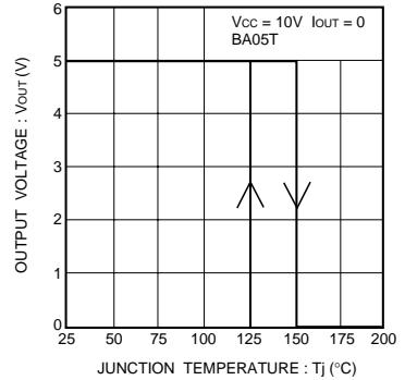
Fig. 8 Thermal cutoff circuit characteristics (BA05T)
