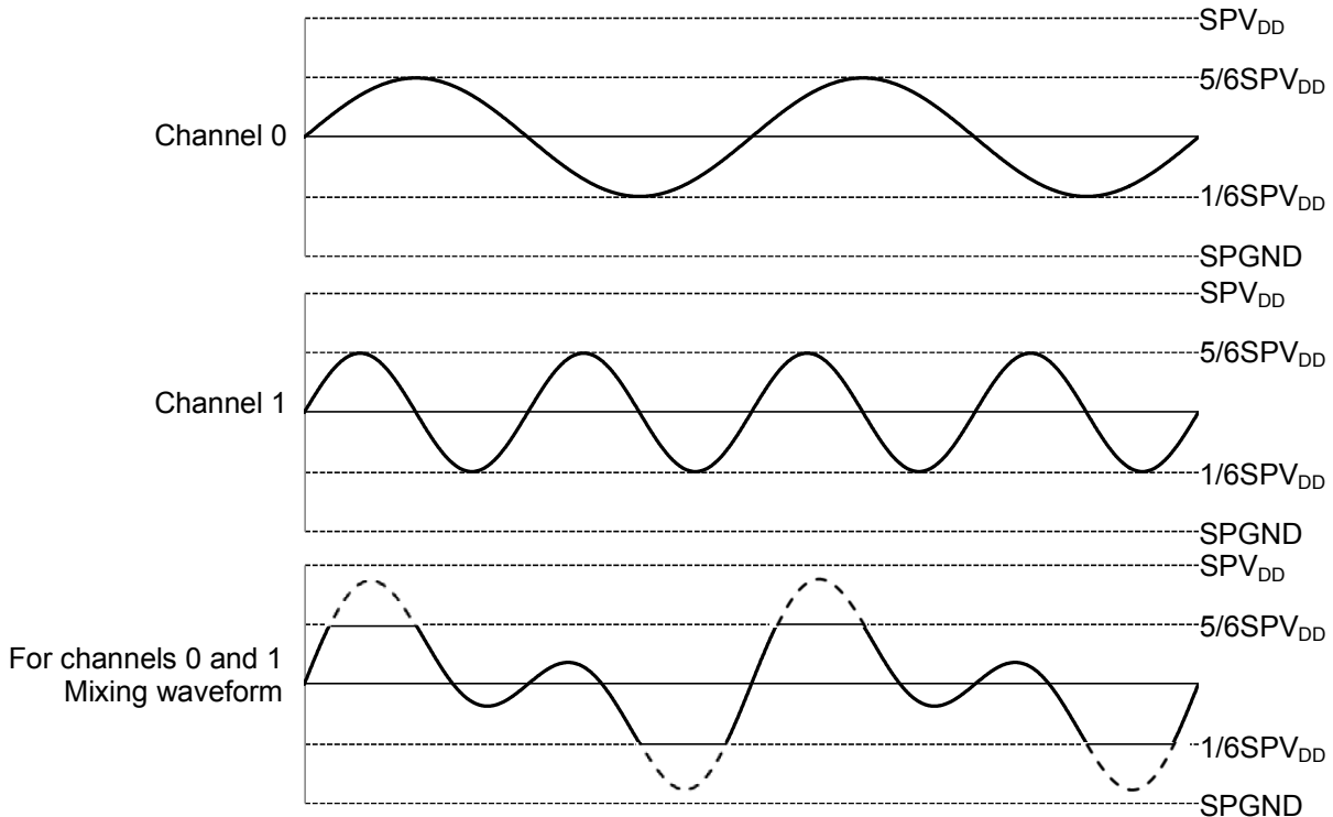
If the result of mixing channels 0 and 1 exceeds from the 1/6SPV_{DD} to 5/6SPV_{DD} level (as indicated by the broken line), the sound quality may be reduced by clamping. Waveforms when AVOL is set to 0.0dB.
