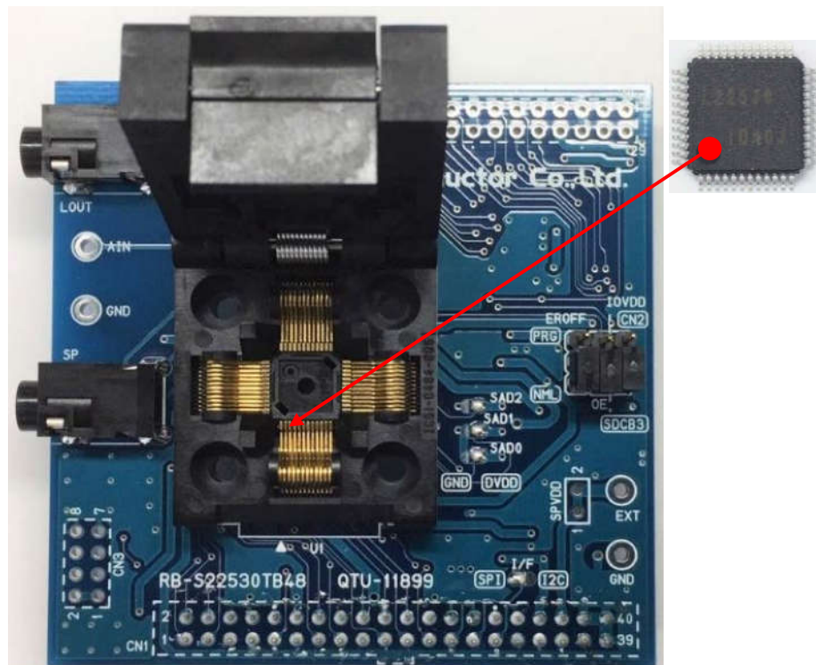
Figure 1 Outline Diagram
