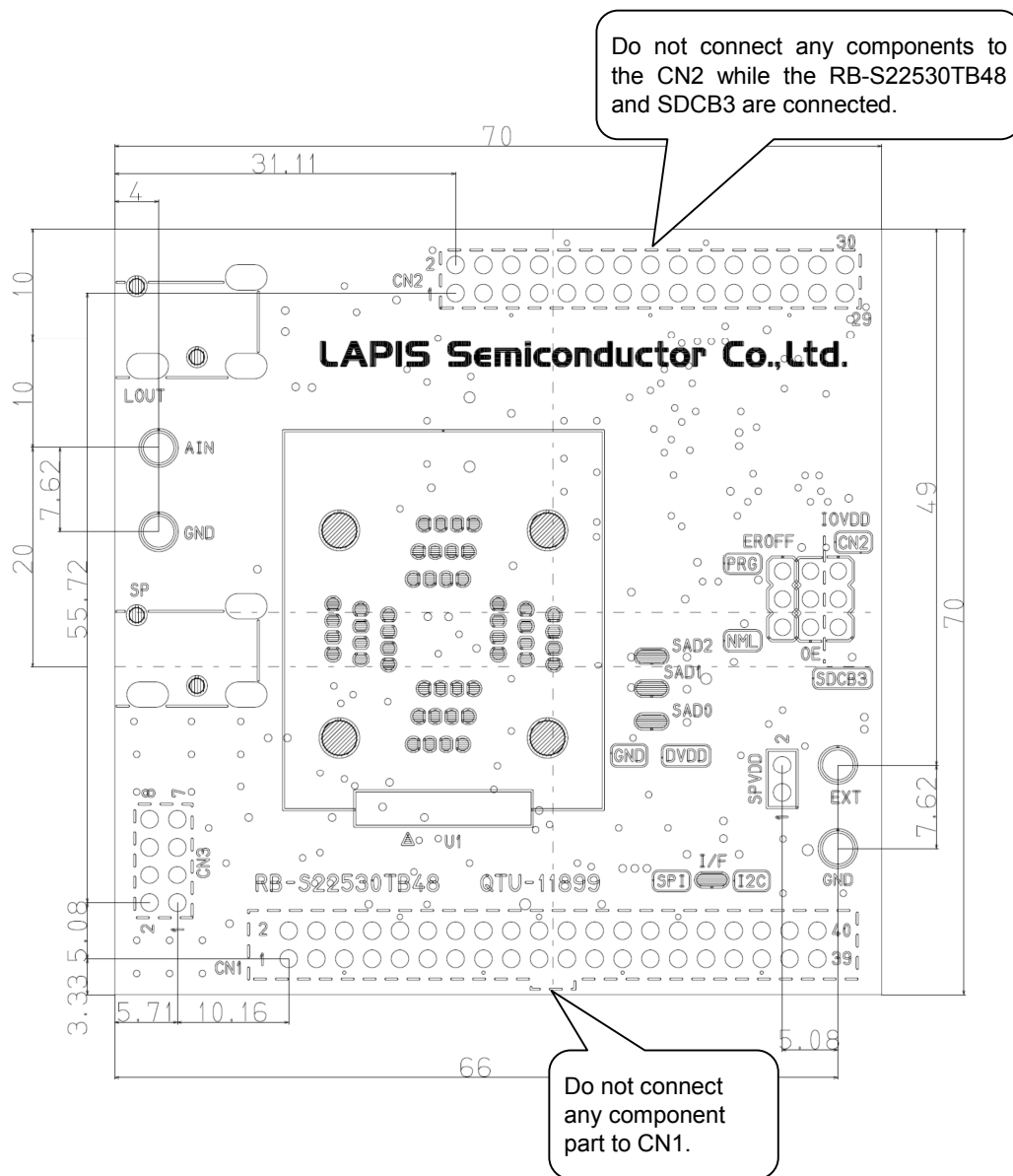
Figure 2 PCB layout
