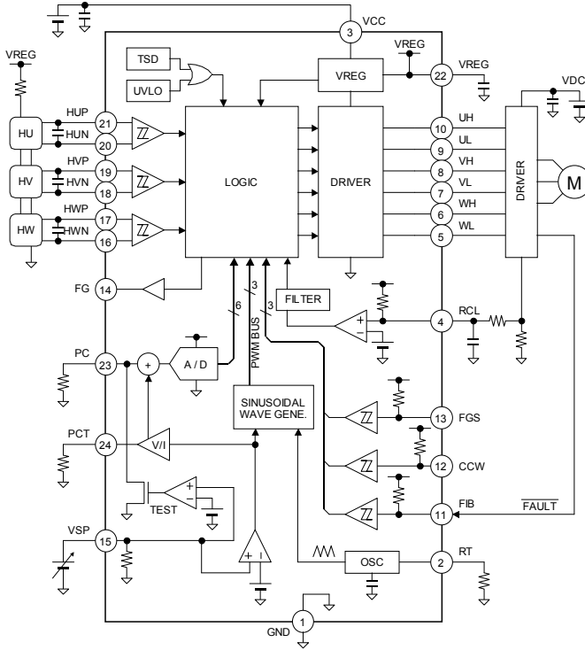
Figure 2. Block diagram
