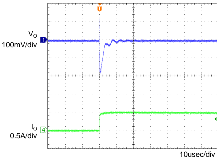
Figure 5. Transient Response (0→0.5A) Co=1μF, Ta=105°C
