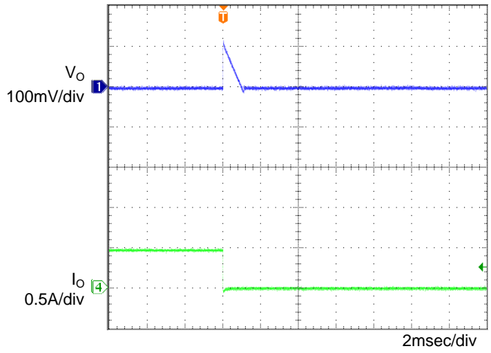
Figure 6. Transient Response (0.5→0A) Co=1μF, Ta=-40°C
