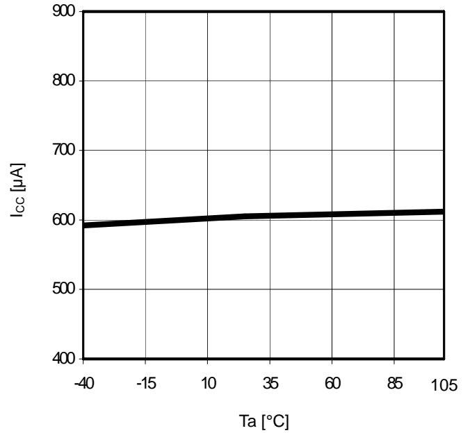
Figure 22. T_a - I_{cc}
