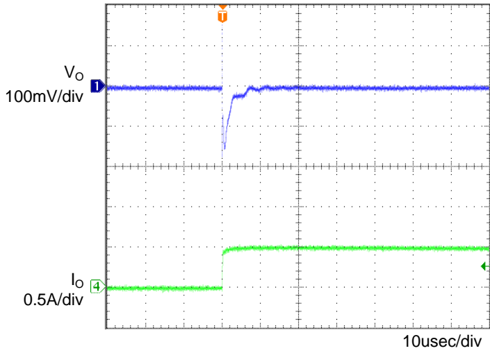
Figure 3. Transient Response (0→0.5A) Co=1μF, Ta=-40°C
