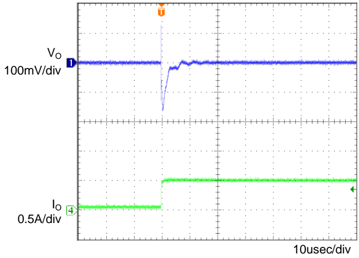
Figure 4. Transient Response (0→0.5A) Co=1μF, Ta=25°C
