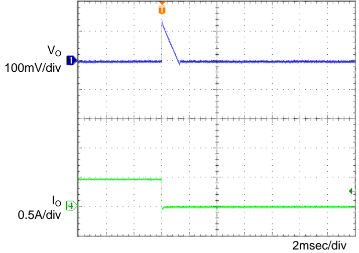
Figure 8. Transient Response (0.5→0A) C_o=1\mu F, T_a=105^\circ C
