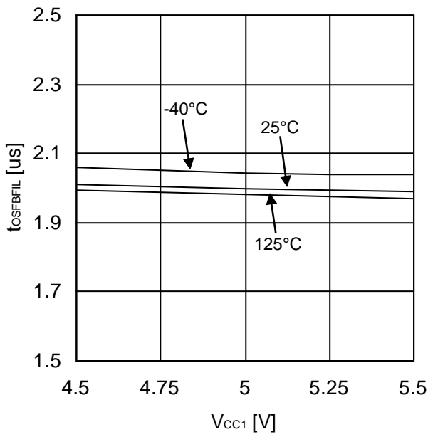
Figure 75. OSFB Output Filtering Time
