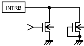
Figure 31. Output circuit (INTRB)
