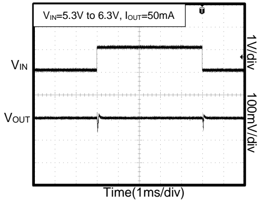
Figure 1. Line-Transient Response
