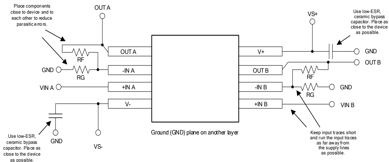
Figure 20. Layout Example
