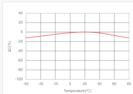
Temperature Characteristics of Capacitance(TCC) LCR meter, 1kHz, 0.27Vrms
