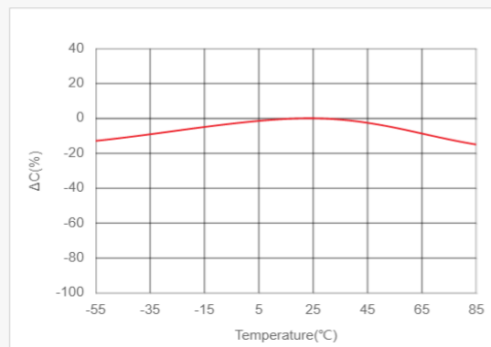
Temperature Characteristics of Capacitance(TCC) LCR meter, 0.12kHz, 0.07Vrms
