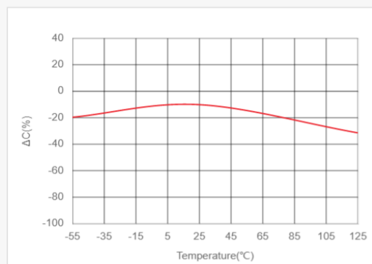
Bias TCC Characteristics LCR meter, 1kHz, 0.5Vrms, 2Vdc
