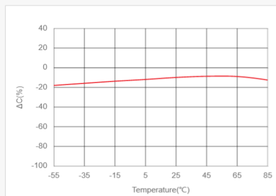
Bias TCC Characteristics LCR meter, 1kHz, 1Vrms, 3.15Vdc
