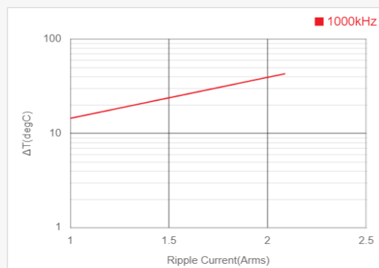
Temperature Rise by Ripple Current 1000kHz
