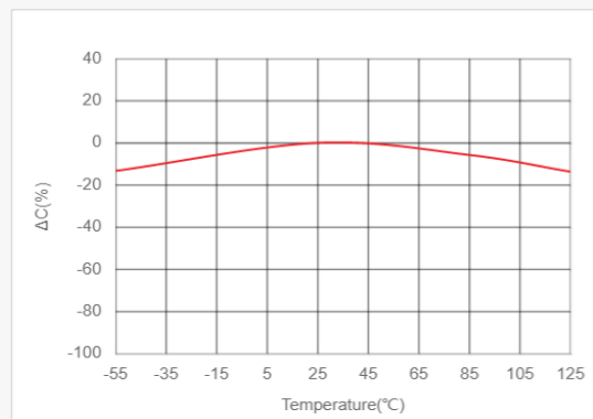
Temperature Characteristics of Capacitance(TCC) LCR meter, 1kHz, 0.05Vrms
