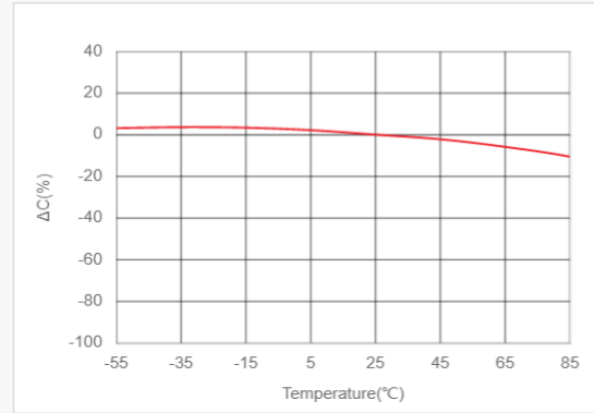
Temperature Characteristics of Capacitance(TCC) LCR meter, 0.12kHz, 0.2Vrms
