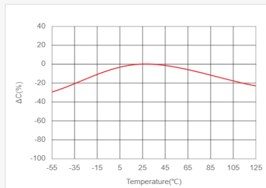
Temperature Characteristics of Capacitance(TCC) LCR meter, 1kHz, 0.02Vrms
