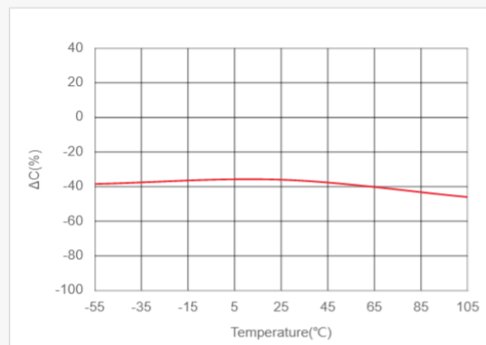
Bias TCC Characteristics LCR meter, 1kHz, 1Vrms, 2Vdc
