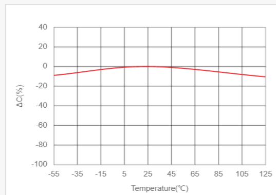
Temperature Characteristics of Capacitance(TCC) LCR meter, 0.12kHz, 0.35Vrms
