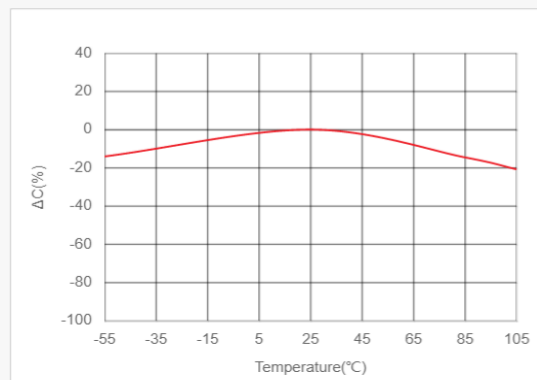
Temperature Characteristics of Capacitance(TCC) LCR meter, 0.12kHz, 0.05Vrms
