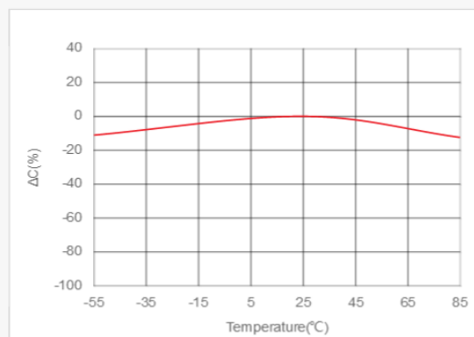
Temperature Characteristics of Capacitance (TCC) LCR meter, 1kHz, 0.12Vrms
