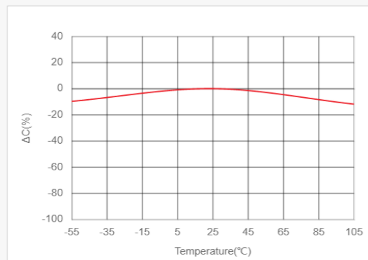
Temperature Characteristics of Capacitance(TCC) LCR meter, 1kHz, 0.3Vrms
