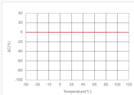
Bias TCC Characteristics LCR meter, 1000kHz, 1Vrms, 8Vdc
