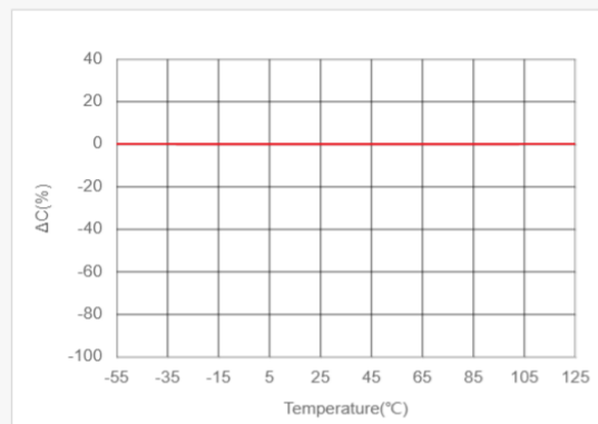
Bias TCC Characteristics LCR meter, 1000kHz, 1Vrms, 40Vdc
